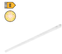
Renton 110 47806101 White | Plastic LED Module 13W | 1450lm | 2700K H: 3,4 cm | W: 2 cm | L: 111,2 cm
